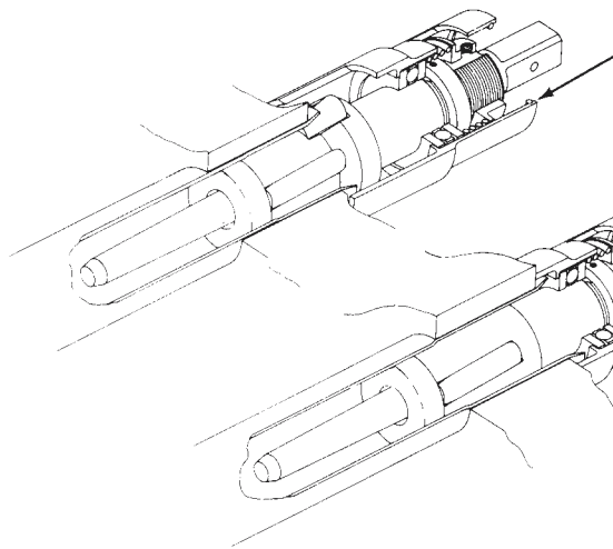
B-2000 EXPANDER AS FIRST OPERATION TOOL IN THICK DRUMS OR TUBE SHEETS
